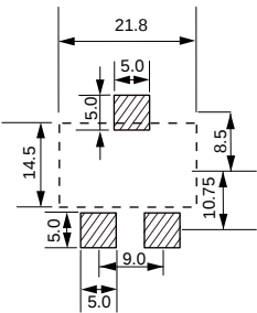
Land Pattern: [mm]
