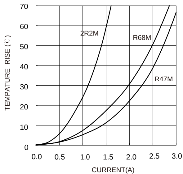
Temp. Rise VS DC Current Characteristics:
