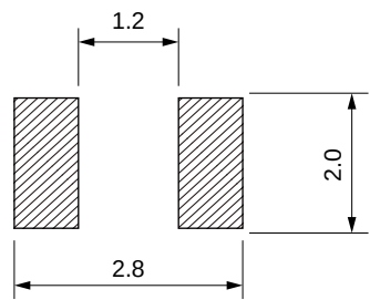
Land Pattern: [mm]
