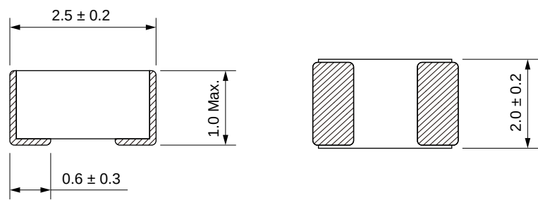
Dimensions: [mm]
