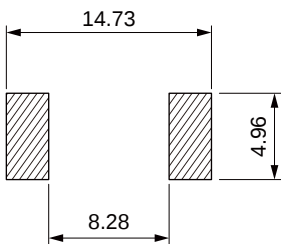
Land Pattern: [mm]
