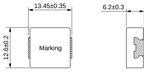
Dimensions: [mm]
